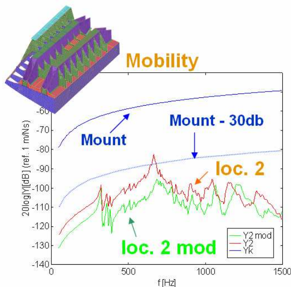
Figure 9: An FE model of the source structural foundation is used to compute input mobility at attachment points. Resilient mount mobilities are compared with structural ones. At least 30 dB difference is required to ensure low level of energy being transmitted to rest of the structure.
