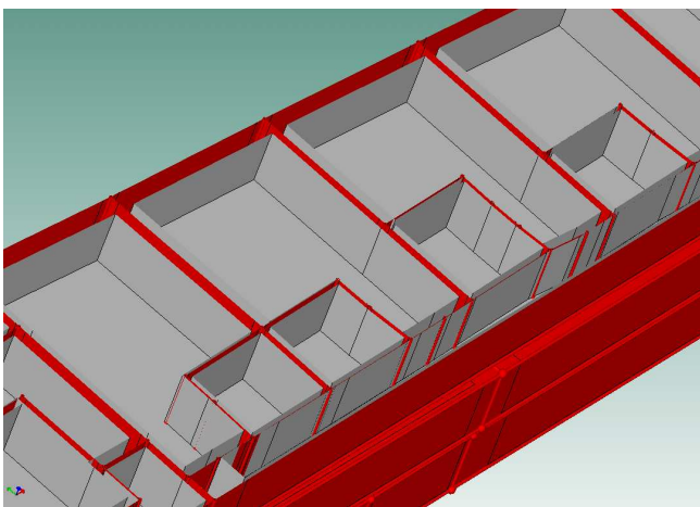
Figure 4: Cabins and tank cavities are created automatically following panel geometry and naming convention. GRAY: cavities (shrunk for visualization), RED: Point, Line and Area junctions [5]
