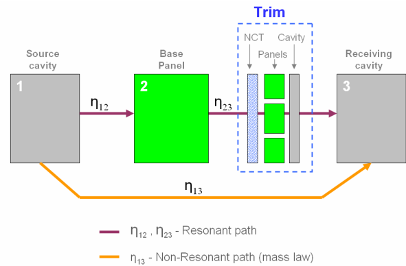
Figure 5: The condensation method replaces the complex trim (foam, fiber, elastic panel, air gap or mass layer combined with structural panels, beams, double wall construction connected with rigid or flexible junctions) by two IL and one damping spectrum.
